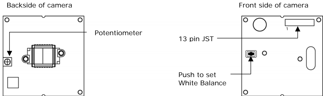
Figure 8. Connectors
