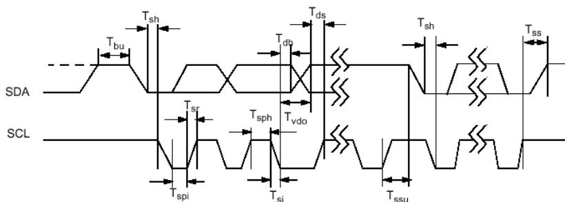
Figure 5. Communication Timing
