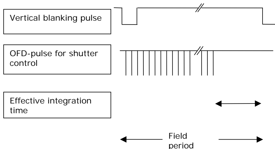
Figure 1. OFD Shutter Control
